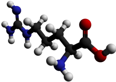
Arginine
